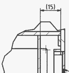
M (1:1)
